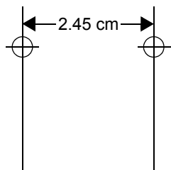
Wall Template for the Charger unit
